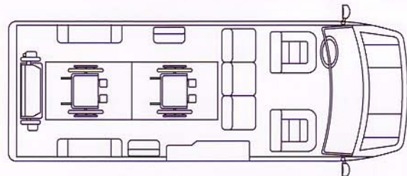
140" WB 6 Passenger/2 Wheelchair plus Driver
