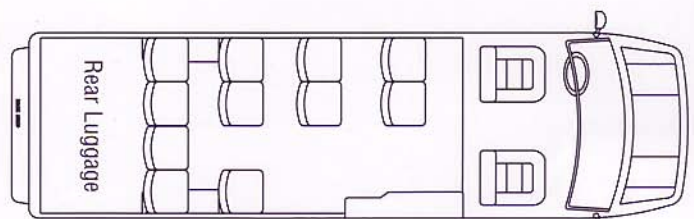
158" WB Sprinter 12 Passenger plus Driver
